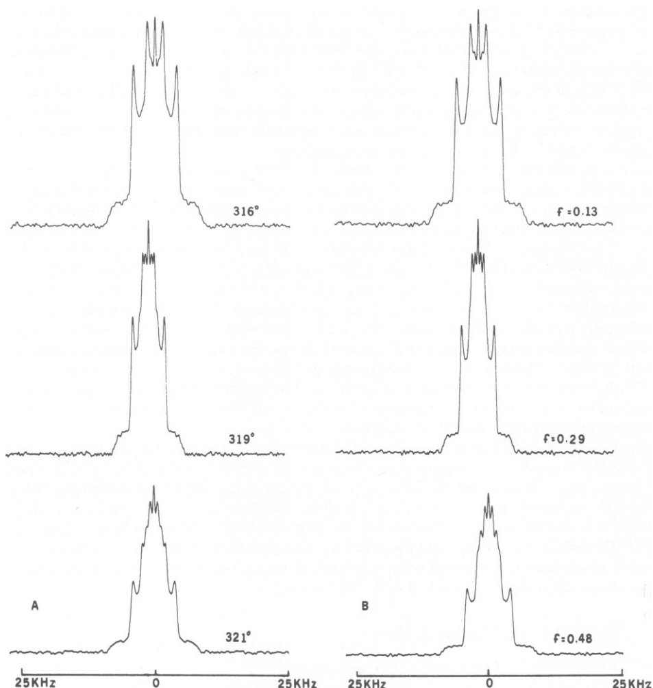
FIGURE 1 (A) ^2\text{H} NMR spectra of phosphatidylethanolamine- \text{d}_4 :cholesterol (4:1) at 46.063 MHz, after accumulating 6,000 scans using the quadrupolar echo technique, and 90^\circ ( 4.5 \mu\text{s} ) pulses. (B) ^2\text{H} NMR spectra simulated by combining spectra obtained at 326^\circ and 310^\circ\text{K} according to the indicated fractions ( f is for the hexagonal-phase fraction).
